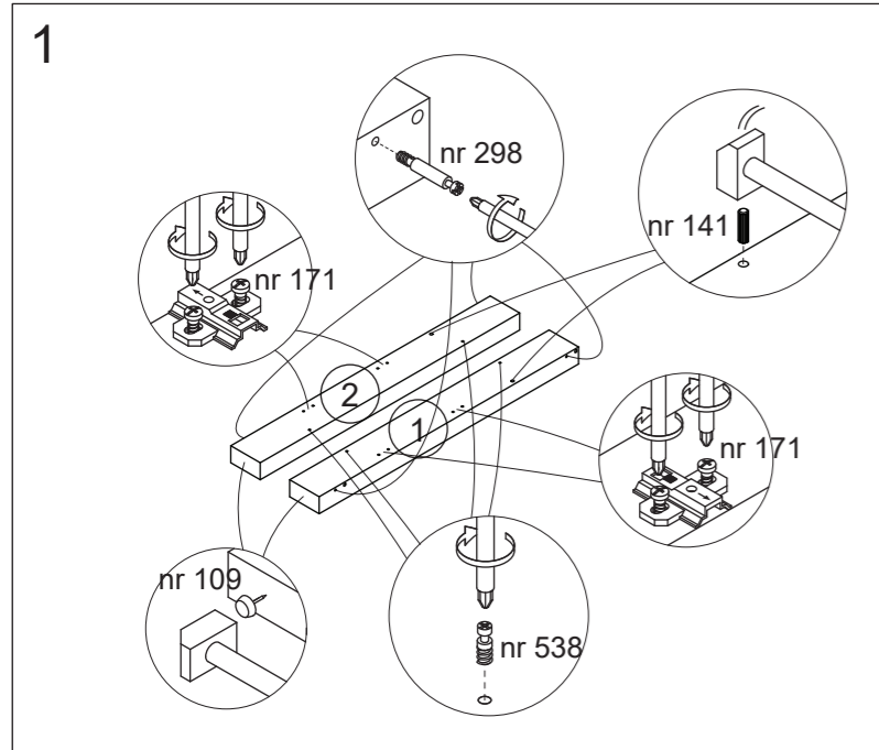
BKO 134 x 89 (96) x 50 (75) cm
