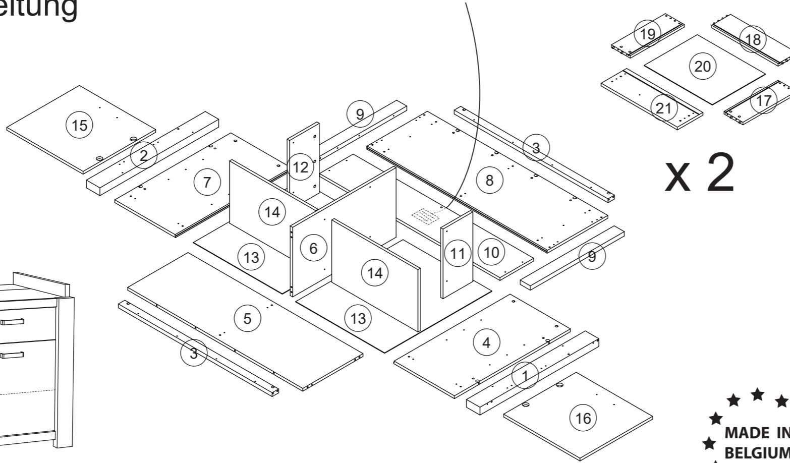
BKO 134 x 89 (96) x 50 (75) cm
